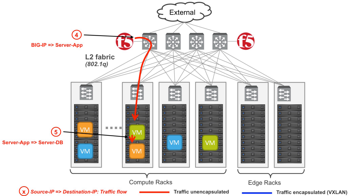
Figure 13. North-south physical traffic flow 2 “Parallel to DLR” with BIG-IP appliances
