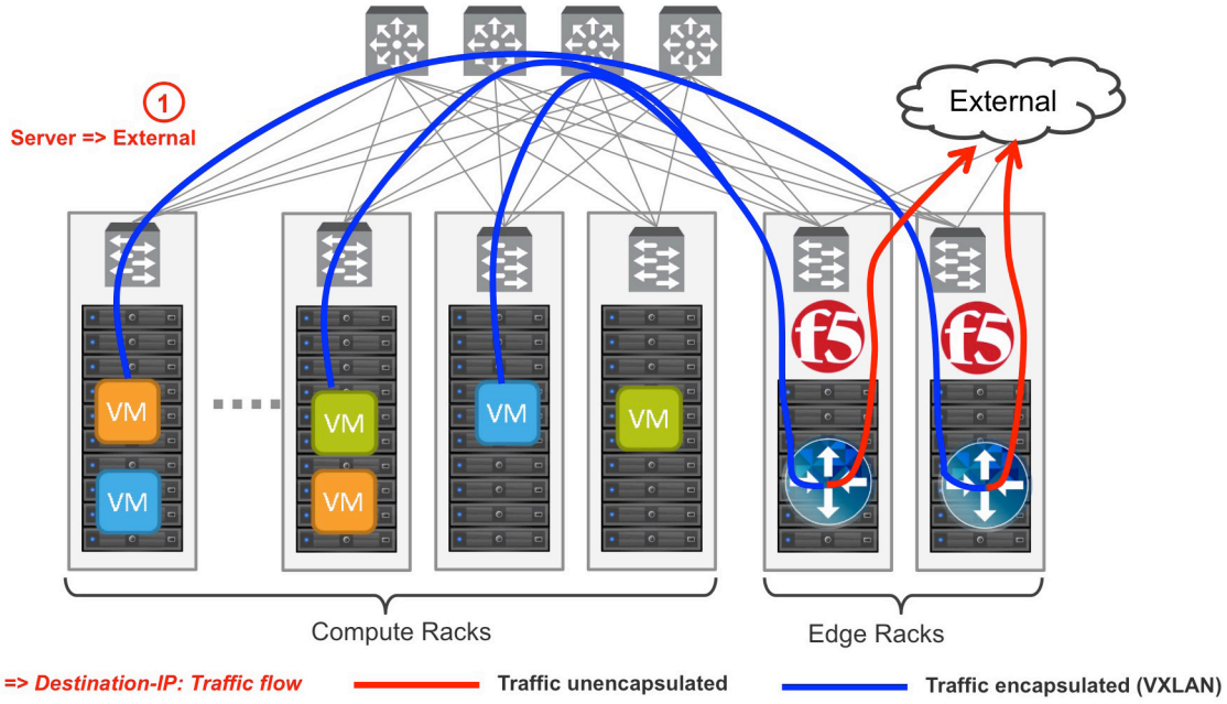
Figure 8. South-north physical traffic flow “Parallel to NSX Edge” with BIG-IP appliances
