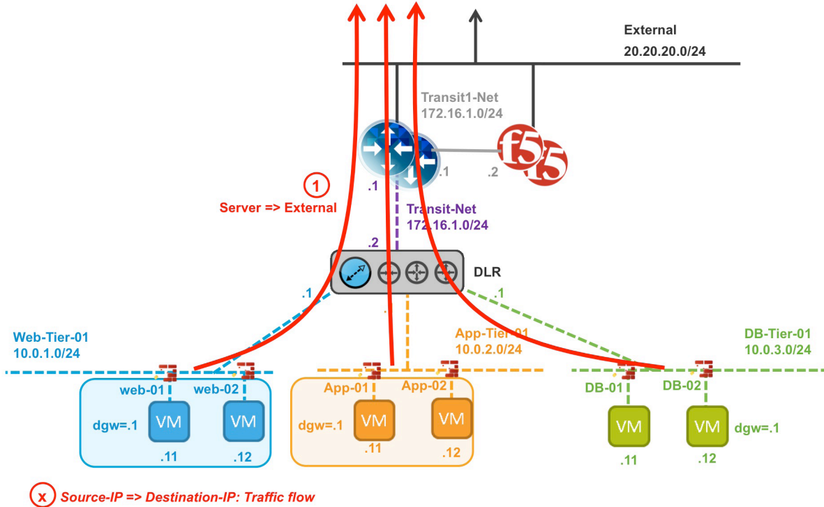
Figure 7. South-north logical traffic flow “Parallel to NSX Edge” with BIG-IP appliances
